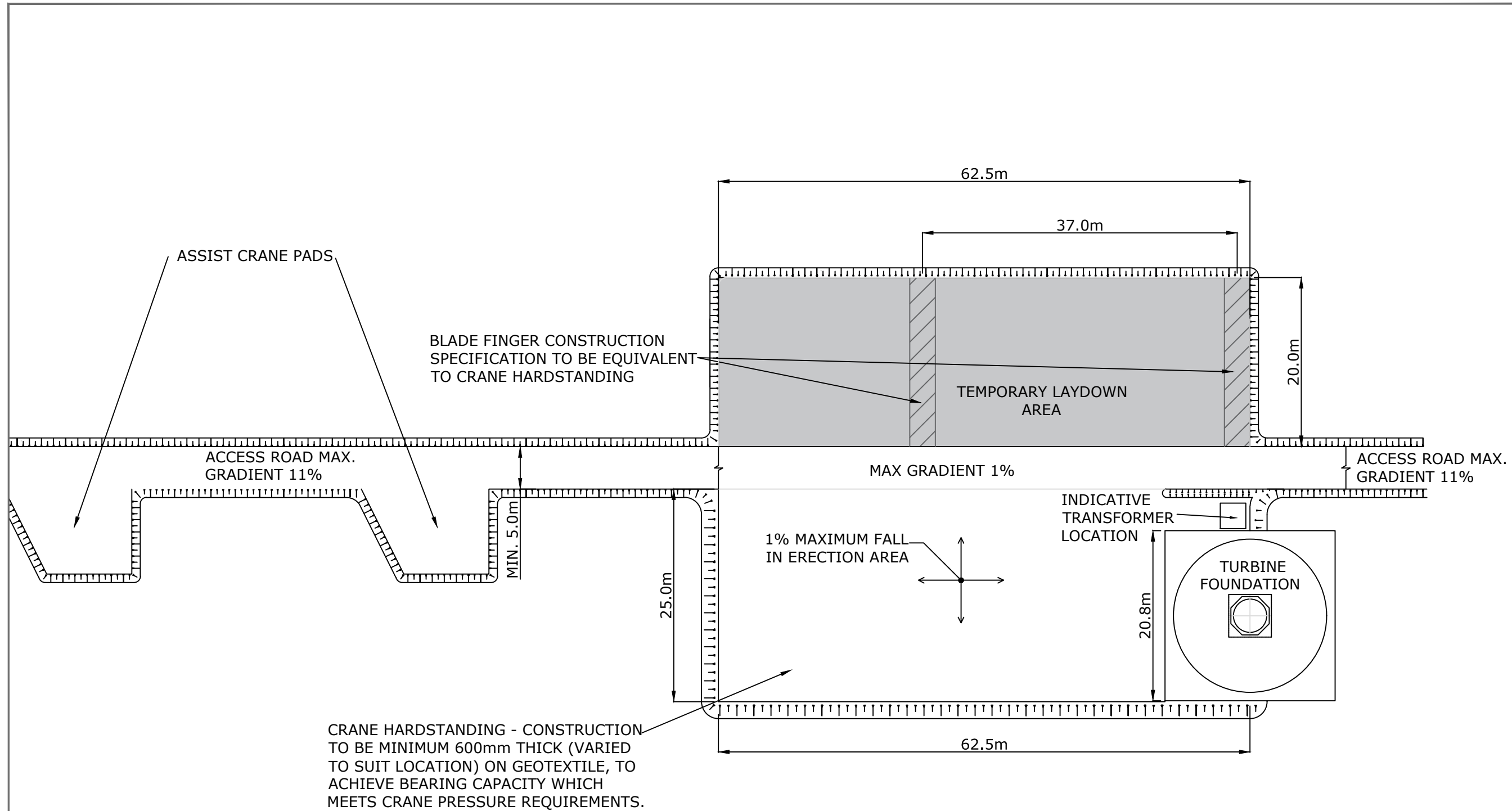
TYPICAL STANDARD CRANE HARDSTAND (1:500)
